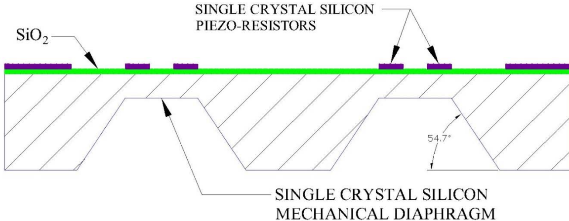
FIG. 1: KULITE SILICON SENSOR CHIP
