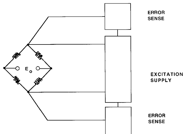
Figure 6-1: 6-Wire Connection to Wheatstone Bridge
